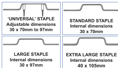
9606 2009 London Bar Frame Reinforcer for lock side 5 staple sizes - std, lge, extra lge, universal & SC71 With countersunk holes for screw fixing
